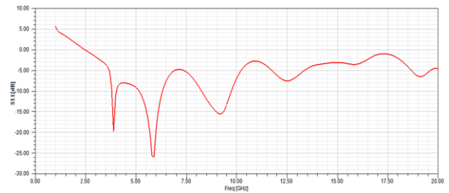
Fig 5 S_{11} parameter of microstrip patch
