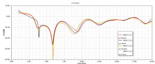
Fig 6 Parametric y dimension variation of microstrip patch
